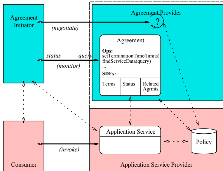
Figure 1: In OGSI-Agreement, agreements are represented as Grid services. Two kinds of operation are provided in the interface of an agreement provider for use by the (client) agreement initiator : anegotiation operations establishe agreements and monitoring operations follows the status of agreements. In the figure, solid arrows point with solid arrowhead towards the invoked service, and with hollow arrowheads towards the client who receives results. Agreement terms are an abstract description of behavior, capturing requirements on the behavior of the application service with respect to a (client) user . The many possible monitoring and effects relationships between components are represented in the figure with dashed, bidirectional arrows; not all such links are necessarily present in every scenario.
