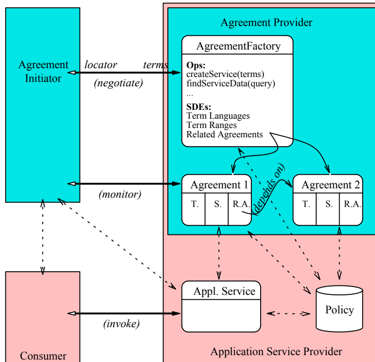
Figure 2: The OGSI-Agreement model uses OGSI service creation as the negotiation primitive, by providing an AgreementFactory interface to agreement providers, inheriting from the ogsi:Factory portType. To support more complex negotiations, OGSI-Agreement allows agreements to be linked by extensible relationships. In this example, Agreement 1 depends on Agreement 2; a common scenario where this might occur is with advance reservation. Agreement 2 represents an advance reservation (future promise) of service capability, and Agreement 1 is an agreement for service exploiting that advance reservation. This scenario illustrates an implementation strategy (for the choice introduced in Figure 1) of tightly integrating the agreement and application service provider functions, where both behaviors share the same policy store.
